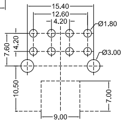
Recommended P.C.B Layout General Tolerance ±0.05
