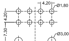
Recommended P.C.B Layout General Tolerance ±0.05
