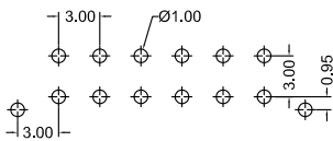
Recommended P.C.B Layout General Tolerance±0.05
