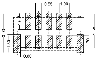
Recommended P.C.B Layout General Tolerance±0.05
